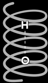
Hydrogen bond before styling (alpha keratin)
