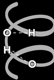
New hydrogen bond created by drying and styling the hair (beta keratin)
