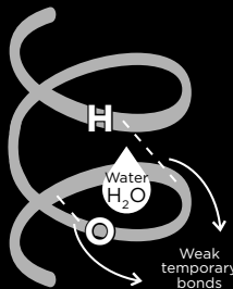
Hydrogen bond broken by water
